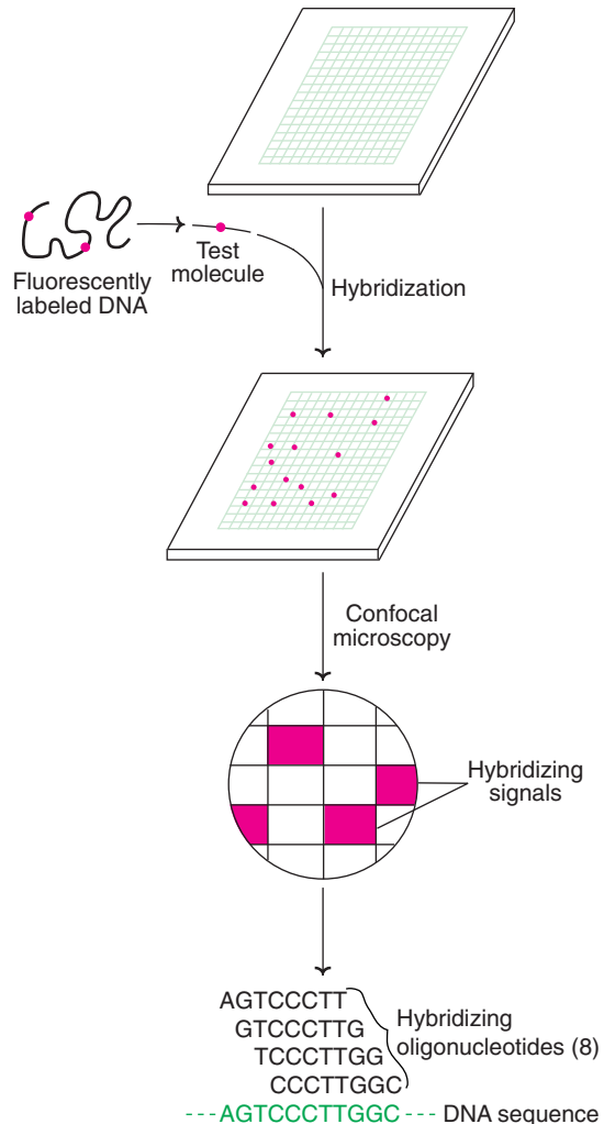
Fig. 27.14 : Microarray (or chip) technology in DNA sequencing.
