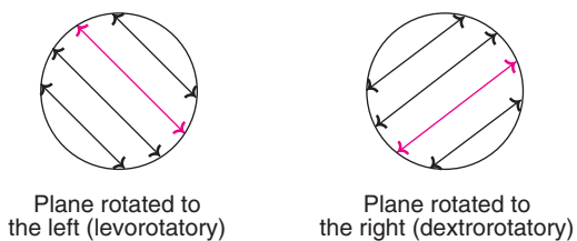
Fig. 39.3 : Diagrammatic illustration of optical activity.
