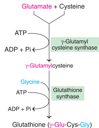
Fig. 15.15 : Outline of glutathione synthesis.
